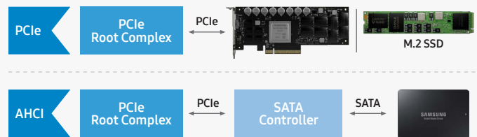
Figure 2. SSD architecture - AHCI versus PCIe interface
