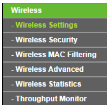
Figure 6-10 Wireless menu
