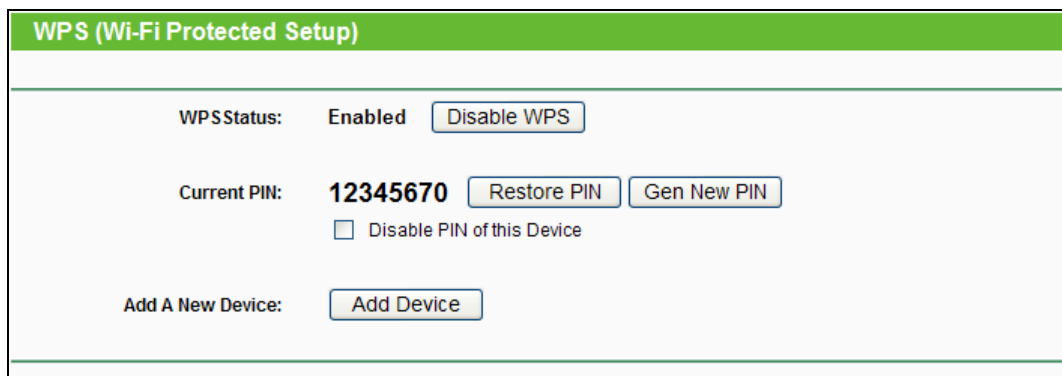
Figure 8-3 WPS
