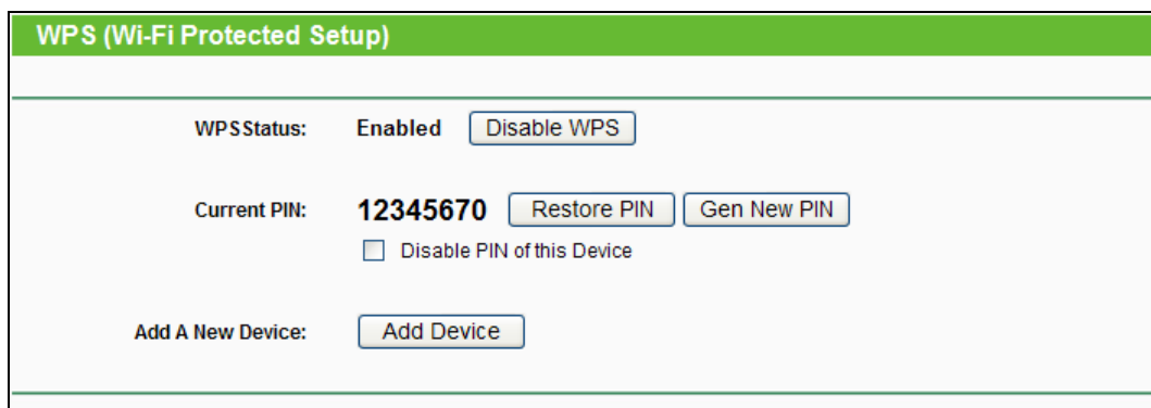
Figure 7-3 WPS
