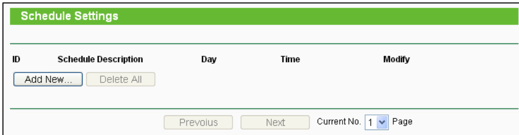
Figure 4-60 Schedule Settings
