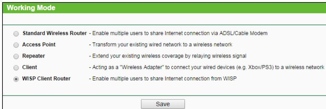
Figure 8-7 Working Mode
