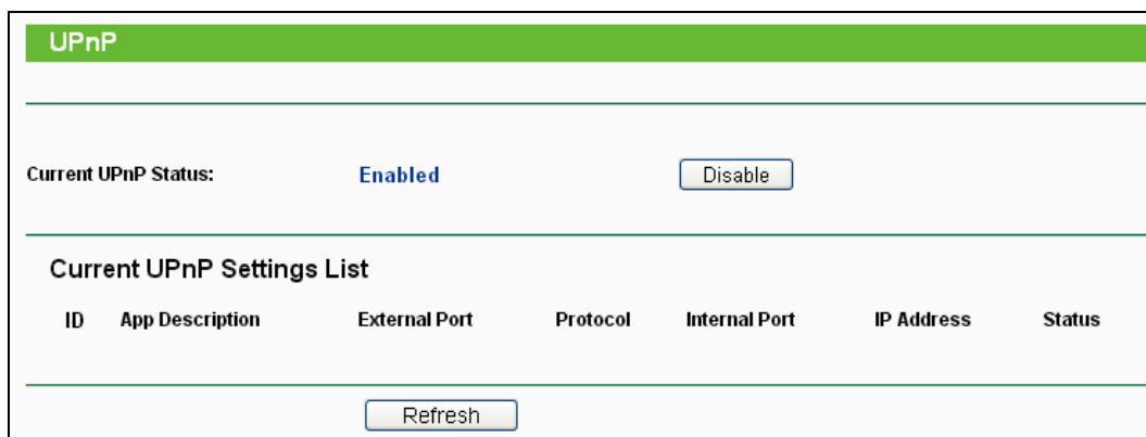
Figure 4-39 UPnP
