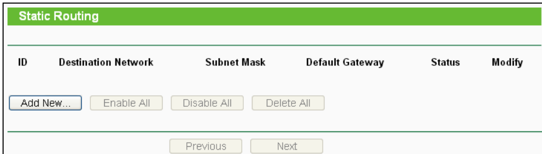
Figure 4-64 Static Routing
