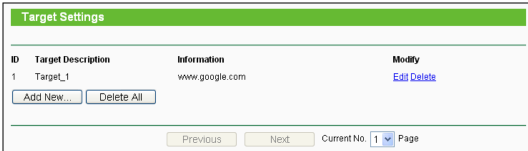
Figure 4-59 Target Settings
