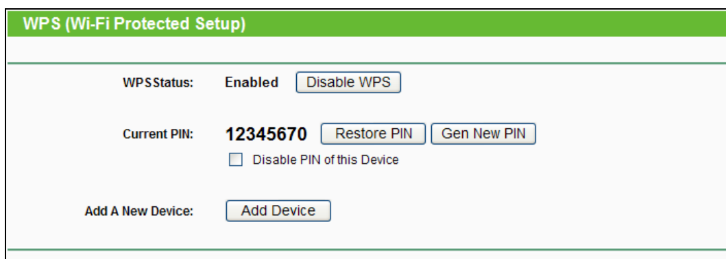
Figure 5-3 WPS
