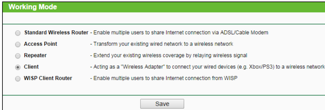
Figure 7-7 Working Mode
