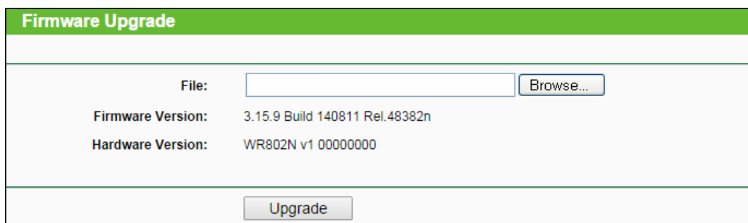
Figure 8-83 Firmware Upgrade
