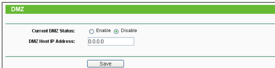
Figure 4-38 DMZ
