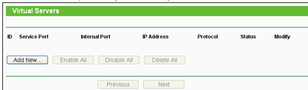
Figure 4-34 Virtual Servers
