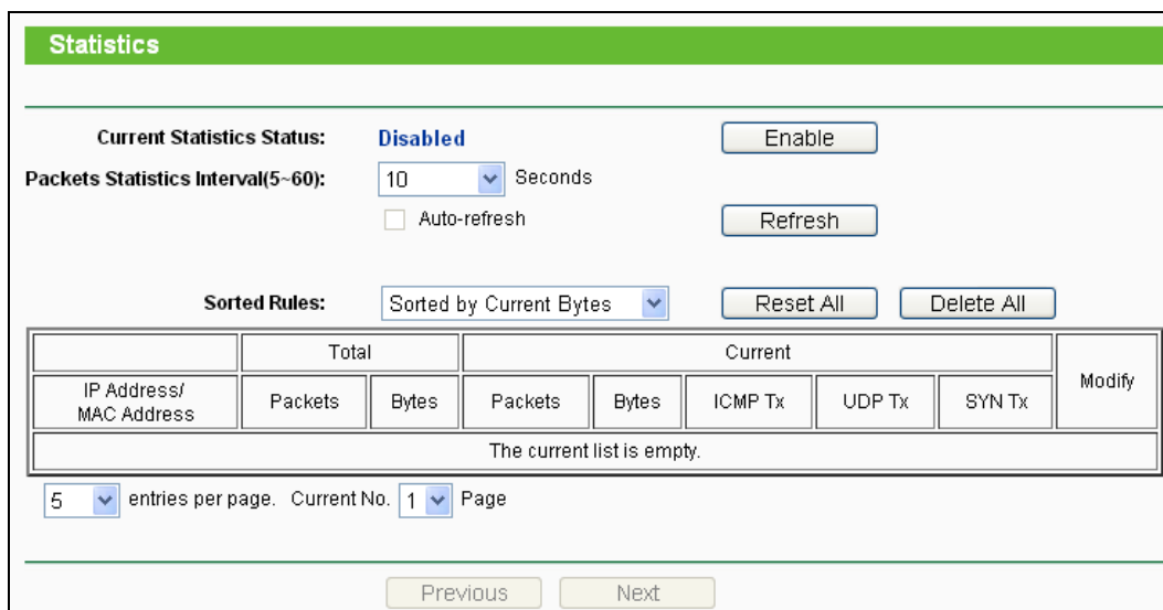
Figure 8-89 Statistics
