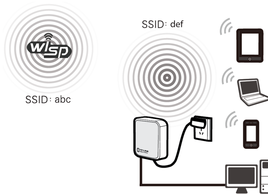
Figure 2-5 Hardware Installation of the TL-WR802N in WISP Client Router Mode
