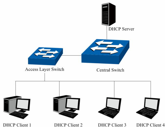
Figure 5-16 Network diagram of DHCP
