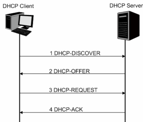
Figure 5-17 Interaction between a DHCP client and a DHCP server
