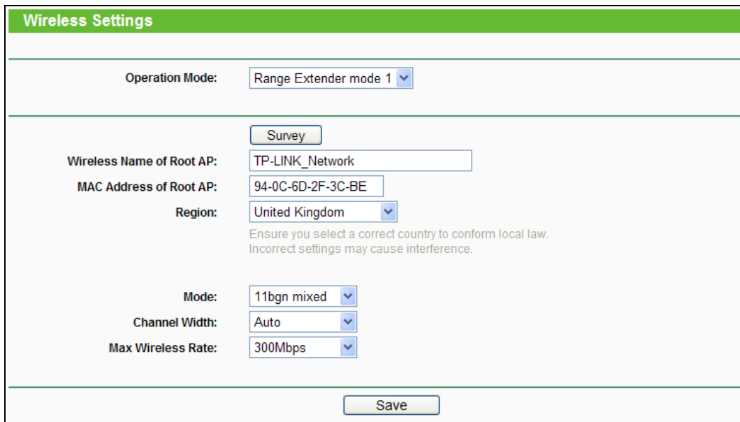
Figure 4-17 Wireless Settings
